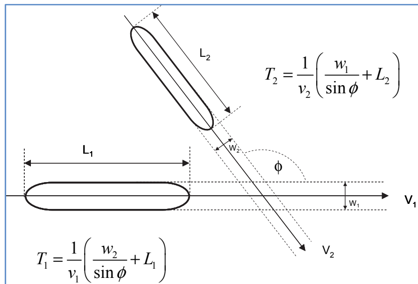
Figure 10. A schematic of a striking ship-struck ship probability model used in the 2005 VTRA.
