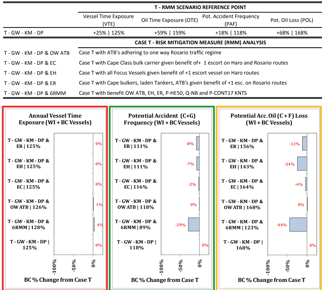
Figure 92. Summary Analysis results of RMM Scenario Analysis enacted on the Combined What-If Scenario (T).
