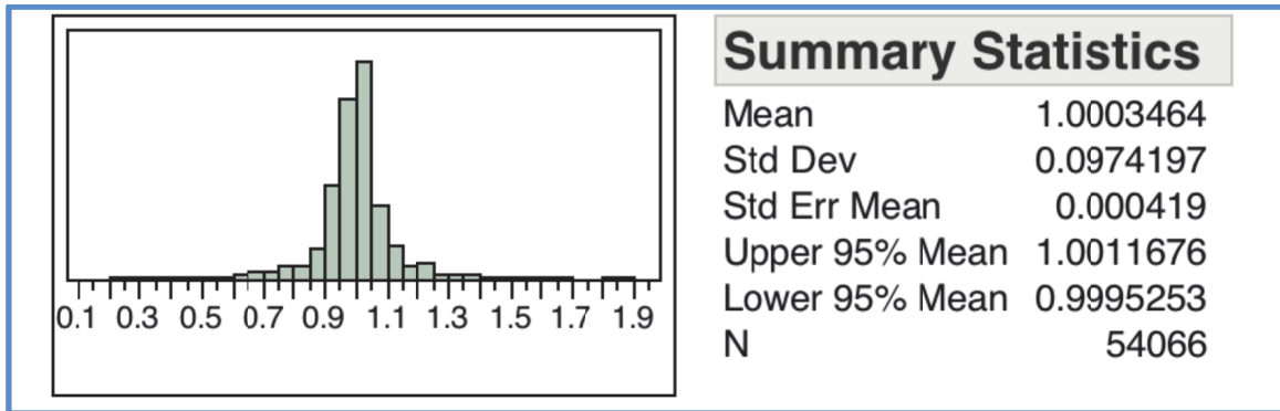
Figure 28. The distribution of the speed accuracy factor for all transits..
