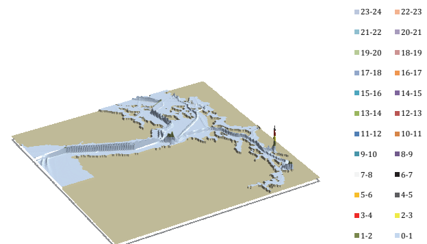
Figure 48. The fuel oil movement density for all focus vessels.
