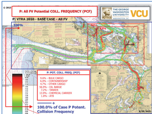
Figure 53. The geographic profile of the POTENTIAL collision frequency.
