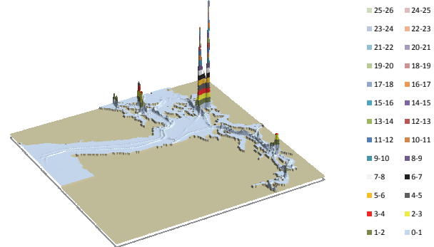
Figure 53. The geographic profile of the POTENTIAL collision frequency.
