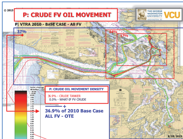
Figure 47. The crude oil movement density for all focus vessels.
