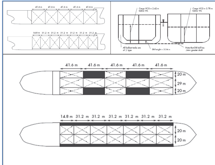
Figure 9. Single hull and double hull 150,000 DWT tanker designs used in 2005 VTRA taken from the National Research Council SR259 report [15].
