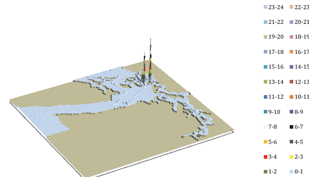
Figure 54. The geographic profile of the POTENTIAL collision oil outflow.
