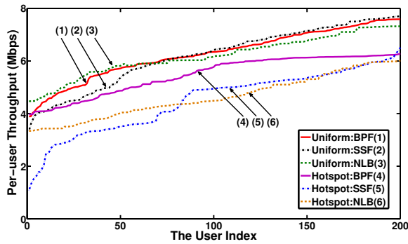
Fig. 5. Per-user Throughput of the Distributed Algorithms in the Dynamic Network Scenario.
