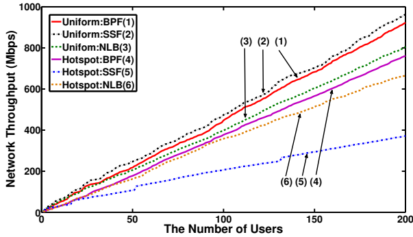
Fig. 4. The Aggregated Throughput vs. the Number of Users.
