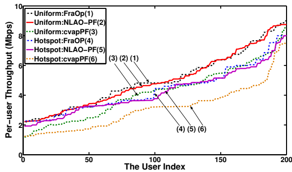
(a) Per-User Throughput of Centralized Algorithms.
