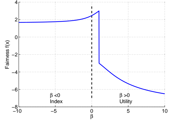
Fig. 1. Plot of fairness f_{\beta}(\mathbf{x}) for different values of \beta : \beta > 0 recovers the utility-based approach, and \beta < 0 recovers the index-based approach.
