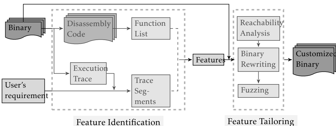
Figure 7. AMASS System Diagram
