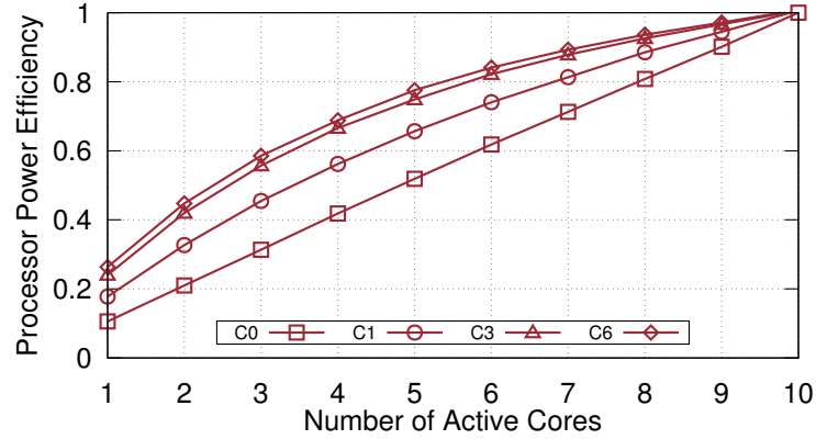
Fig. 2: Power efficiency of a 10-core Xeon processor with different level of C state configurations.
