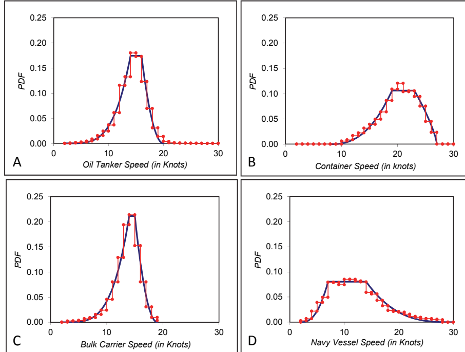
Figure 12. Example representative speed distribution for oil tankers (A), container vessel (B), bulk carriers (C) and navy vessels (D) estimated from VTOSS 2005 data. Step functions indicate the empirical probability distribution functions (pdf), whereas the solid lines are fitted Generalized Trapezoidal Distributions (GTD)[18].
